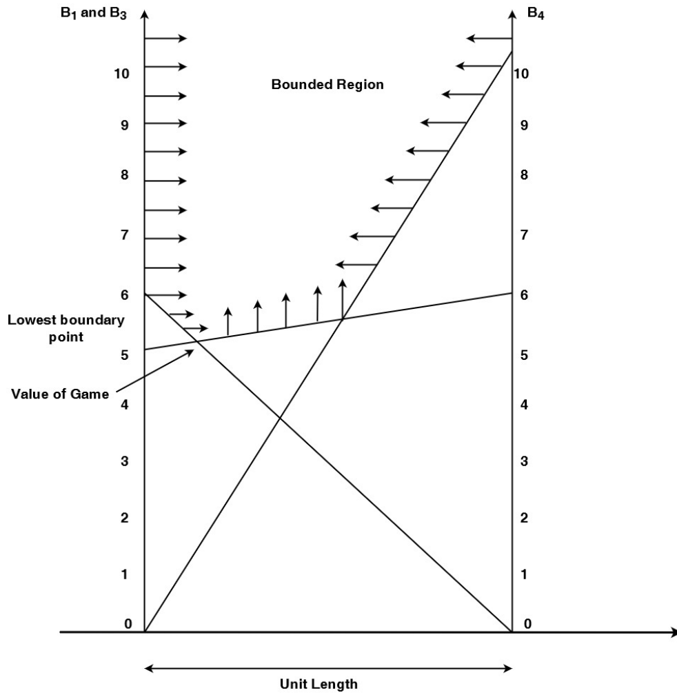
Fig. 17. Graphical representation for third step of dominance property.
