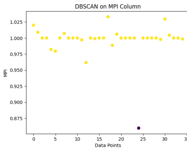
Fig. 4. DBSCAN result.
