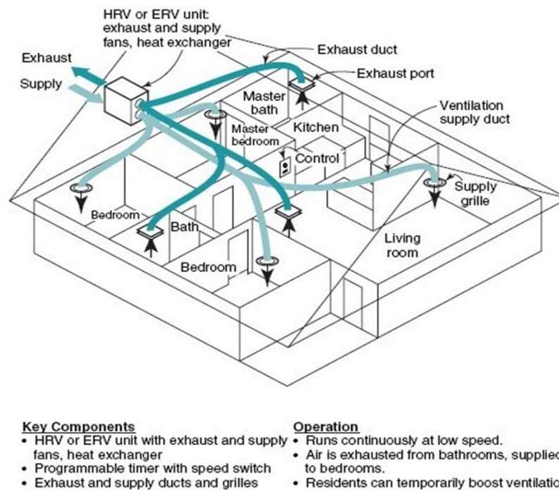
Fig. 3. Balanced ventilation system [42].
