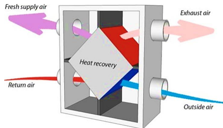
Fig. 4. Heat recovery ventilation system [44].
