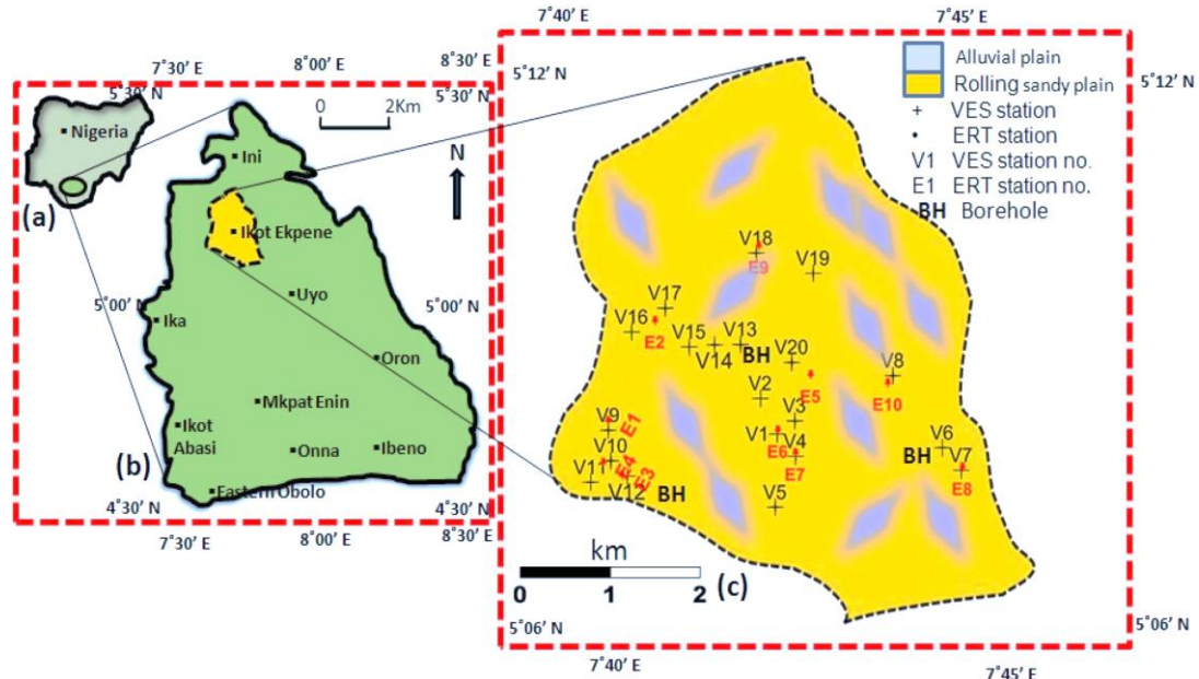
Fig. 1. Map of a Nigeria showing Akwa Ibom State in southern Nigeria, b Akwa Ibom State showing the study area, and c study area showing its geology and sounding stations.
