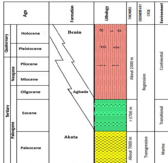
Fig. 3. A schematic diagram showing the general Stratigraphy of the Niger Delta, where the study area is located [29].
