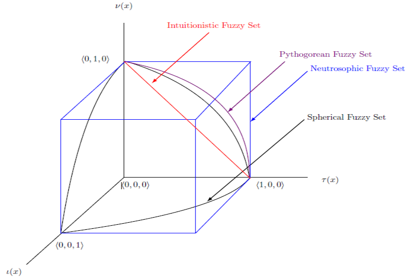
Fig. 1. Geometric representation of fuzzy set and its extension sets.
