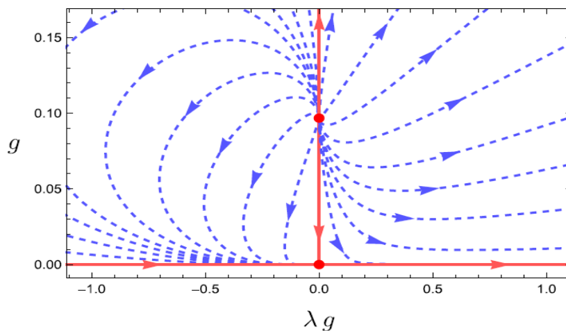
Fig. 4. The one-loop phase diagram of quantum gravity.
