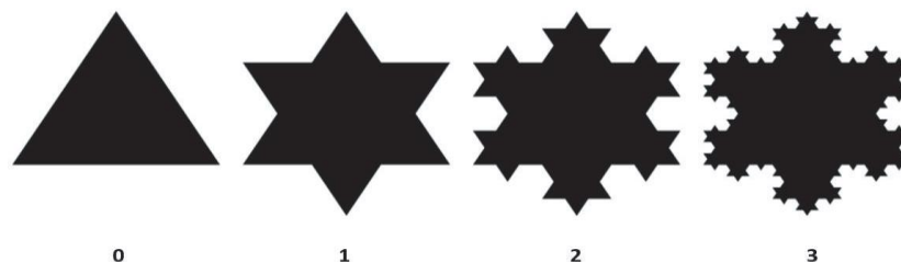
Fig. 3. Expanding Koch snowflake Fractal pattern layers.
